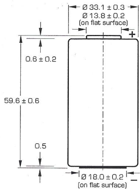
Finished version with flat positive end cap
